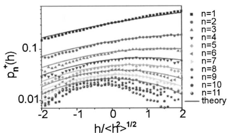
FIG. 5. The spatial p_n^+(h) as a function of h for a number of n for statepoint IV. The drawn lines are the theoretical values.
