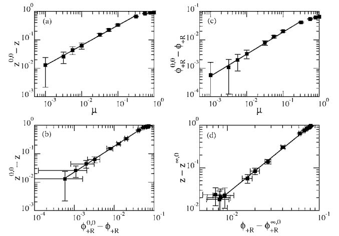
FIG. 4. Scaling of the zero pressure, extrapolated, contact numbers, and packing densities with the friction coefficient \mu . The extrapolated values at zero (infinite) friction are labeled as 0,0 ( 0,\infty ). (a)–(c) When \mu \rightarrow 0 and p \rightarrow 0 , z approaches z^{0,0} \approx 3.975 [20], while \phi_{+R} approaches \phi_{+R}^{0,0} \approx 0.8395 [5]. For finite but small \mu , z and \phi_{+R} appear to scale as (a) (z^{0,0} - z) \sim \mu^{0.70} [10] and (b) (\phi_{+R}^{0,0} - \phi_{+R}) \sim \mu^{0.77} [10]. (c) The contact number and packing deviate similarly from this scaling when \mu approaches 1, and so (z^{0,0} - z) \sim (\phi_{+R}^{0,0} - \phi_{+R})^{0.91} [10]. (d) In the limit of infinite friction and zero pressure, z approaches z^{\infty,0} = 3.00 [2], while \phi_{+R} approaches \phi_{+R}^{\infty,0} = 0.758 [10]. The deviations from these limiting values also appear to be related by a scaling relation of the form (z - z^{\infty,0}) \sim (\phi_{+R} - \phi_{+R}^{\infty,0})^{1.7} [2].
