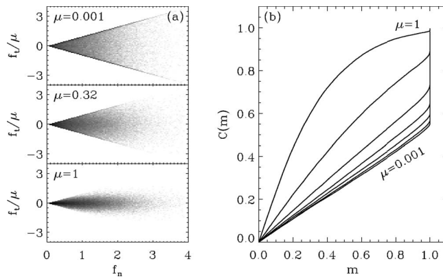
FIG. 2. Mobilization at p=2 \times 10^{-5} . (a) Scatter plots of f_t/\mu versus f_n for three packings at \mu=0.001 , 0.32, and 1. The probability density of normalized tangential ( f_t/\mu ) and normal ( f_n ) forces exhibits a singularity on the Coulomb cone for small \mu , which rapidly diminishes for larger \mu (all forces are normalized so that \langle f_n \rangle = 1 ). (b) The cumulative distribution of the mobilization C(m) \equiv \int^m dm' P(m') exhibits a clear jump near m=1 . Data shown here are for \mu=10^0, 10^{-0.5}, 10^{-1}, \dots, 10^{-3} .
