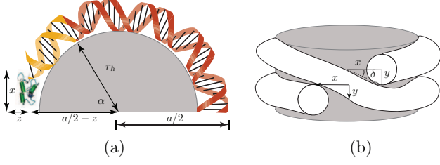
Fig. 3: (Colour on-line) (a) Half-nucleosome with the nucleosomal DNA (red), the stem (orange), and the linker histone (green). Here r_h = 3.75 nm and \alpha = 0.33\pi . (b) A cartoon of the nucleosome from another perspective. For simplicity, the linker histone is omitted. x and y are the distances between the centerline of the DNA and the dyad axis of the nucleosome.
