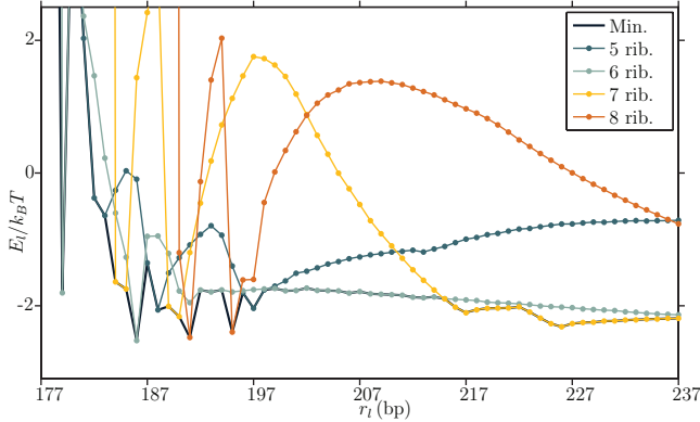
Fig. 5: (Colour on-line) Energy E_l per linker, eq. (3), as a function of repeat length r_l for the four possible N_{\text{rib}} . We assume infinitely long fibers with E_{\text{stack}} = -3k_B T and (x, y, z) = (2.5, 0.5, 0.1) nm. We note that changes in the helicity of the fiber manifest themselves in kinks, as for the 7-ribbons structure at 222 bp (see also fig. 1).
