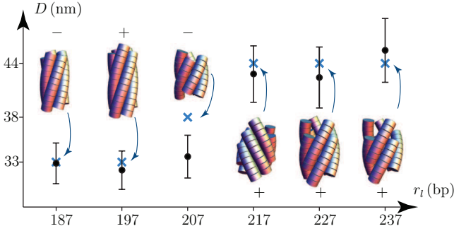
Fig. 1: (Colour on-line) Fiber diameter as function of repeat length: experimental data [4] in black, our theoretical prediction for (x, y, z) = (2.5, 0.5, 0.1) nm in blue.
