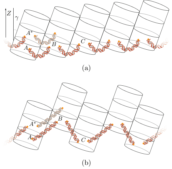
Fig. 4: (Colour on-line) The 5-ribbon fiber rolled out in a plane, omitting the wrapped DNA in the figure for clarity. (a) A constant vertical offset b \cos \gamma / N_{\text{rib}} between connected nucleosomes (e.g., A - B ) leads to highly bent linkers. (b) A zig-zag geometry with vertical offsets \Delta_{\uparrow} for A - B and \Delta_{\downarrow} for B - C can have nearly straight DNA linkers, except close to the entry/exit points where we assume denaturation. Note that the fiber connectivity does not change from (a) to (b) and that the Z -axis indicates here the axis of the fiber and is not related to the z in fig. 3.
