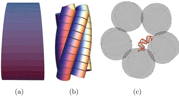
Fig. 2: (Colour on-line) (a) Side view of a nucleosome with the \beta = 8.1^\circ -wedge angle. The DNA leaves the nucleosome on the top. (b) Fiber made from 5 stacks of nucleosomes, N_{\text{rib}} = 5 . (c) Cross-section of (b) showing one of the DNA linkers. In this example nearest stacks are connected, N_{\text{step}} = 1 and the wrapped portion of DNA is hidden for clarity.
